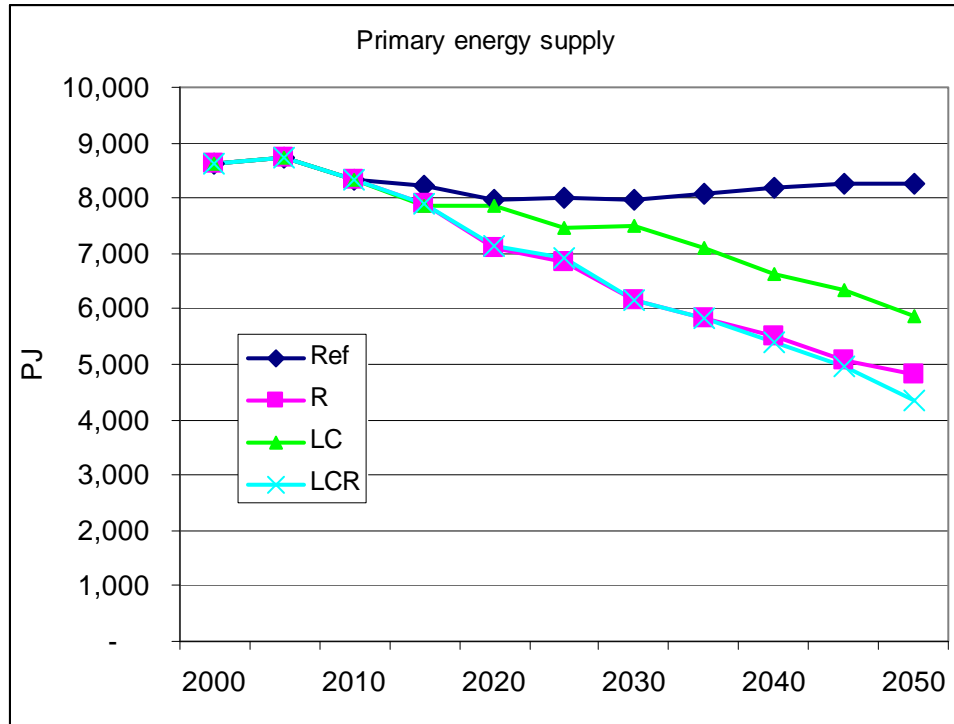
Figure B-1: Trend in primary energy supply in the core scenarios
