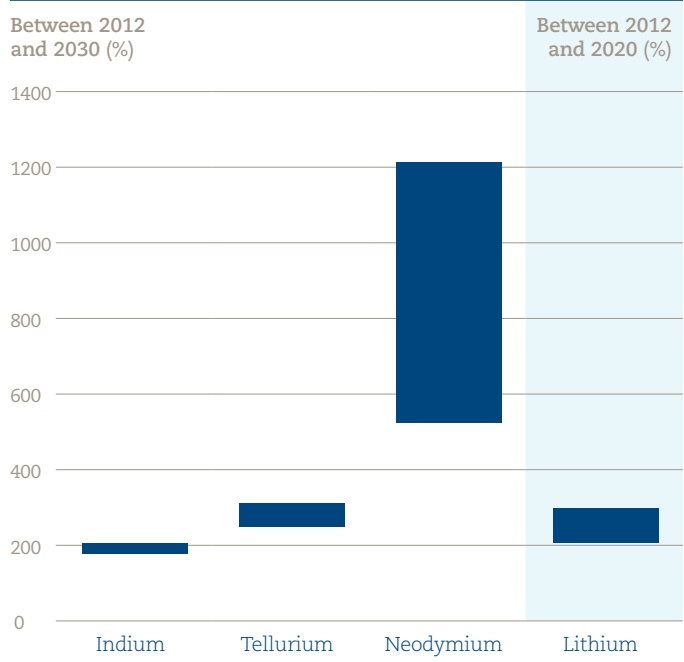
Figure 14: Estimated supply growth by 2030 for indium, tellurium, neodymium and lithium as a percentage of supply in 2012
